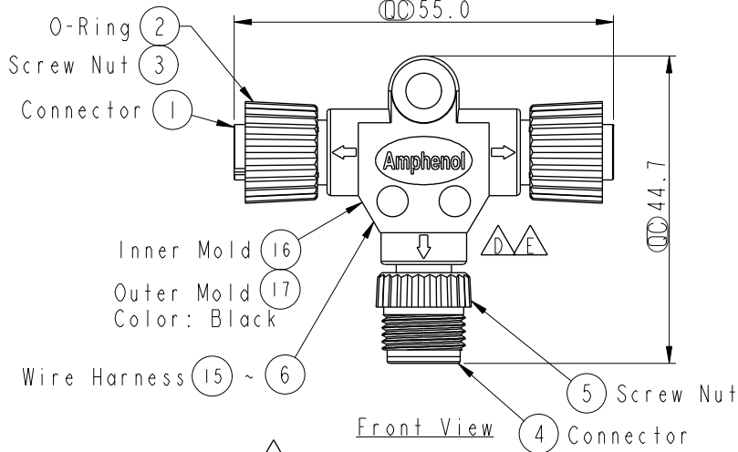
Conn. 3
