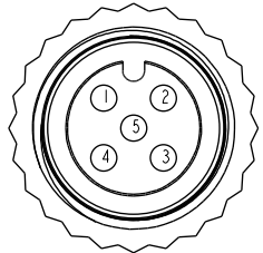
Conn. 2&3 Pin Assignments Front View
