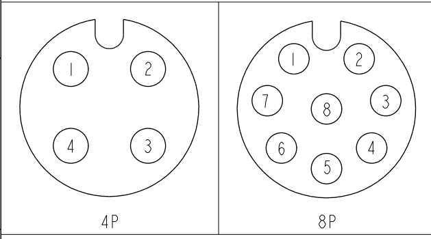
Pin Assignments Front View
