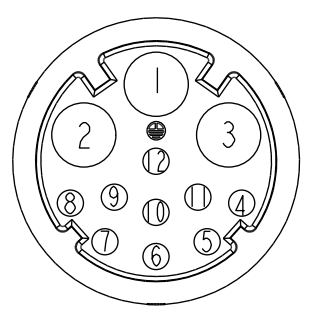
C2 Pin Assignments Front View
