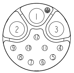
C1 Pin Assignments Front View
