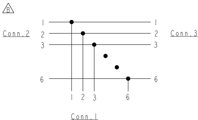
Connection Diagram
