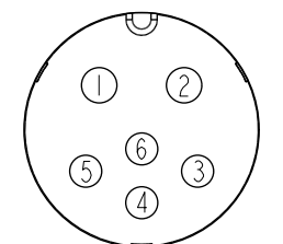
C1 Pin Assignments Front View
