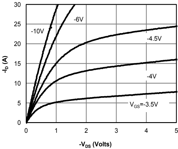
Fig 1: On-Region Characteristics
