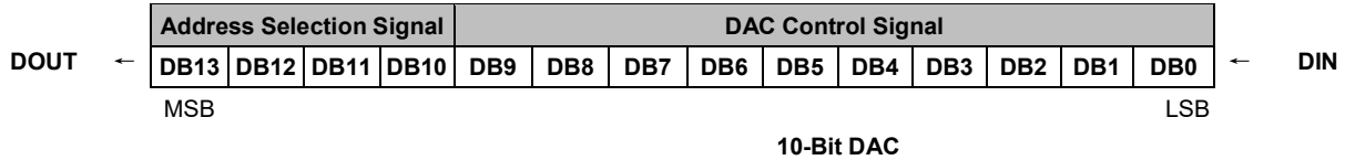
Figure 2. Serial Data
