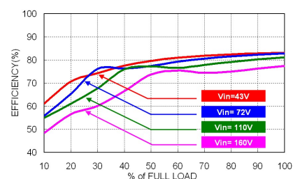
RDL03-110S05W Efficiency vs. Output Load
