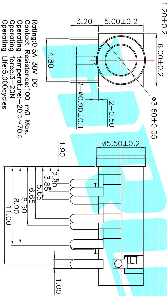
P C B Layout(copper-sided view)
