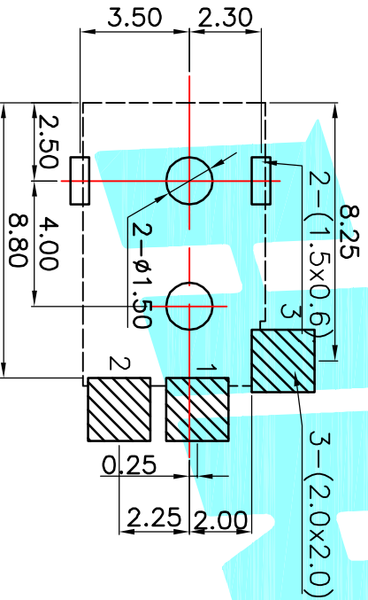
P.C.B LAYOUT(Copper-side view)
