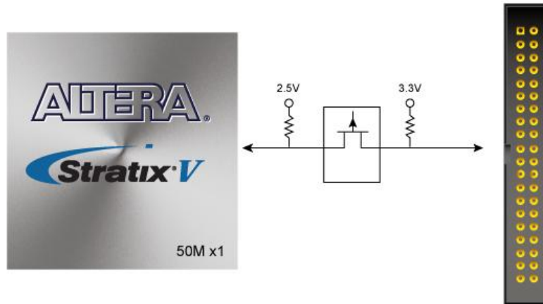
Figure 2-21 Connections between the GPIO connector and Stratix V GX FPGA
