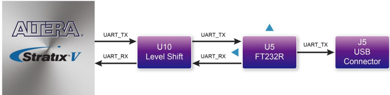
Figure 2-8 Connection between UART-To-USB and Stratix V GX FPGA
