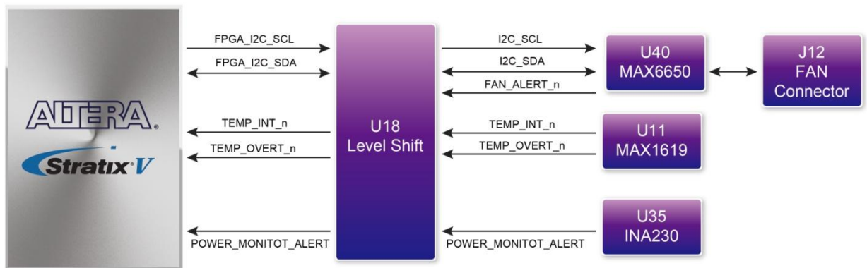
Figure 2-10 Connections between the temperature sensor/fan control/power monitor and the Stratix V GX FPGA
