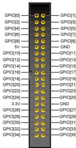
Figure 2-20 GPIO Pin Arrangement
