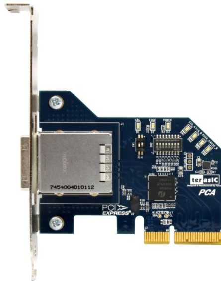
Figure 2-22 PCIe Cabling Adaptor(PCA) card
