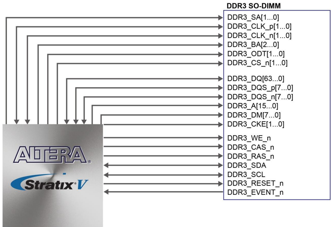
Figure 2-13 Connection between the DDR3 and Stratix V GX FPGA
