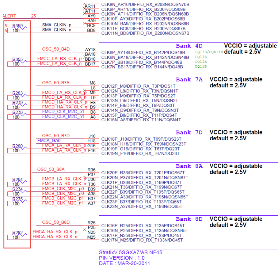
Figure 2-17 Termination resistors on FMC clock I/Os
