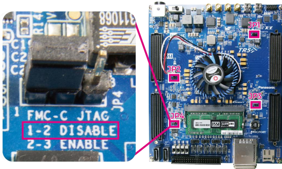
Figure 2-7 FMCC JTAG Header
