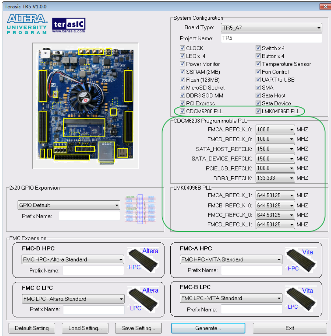
Figure 3-5 External Programmable PLLs
