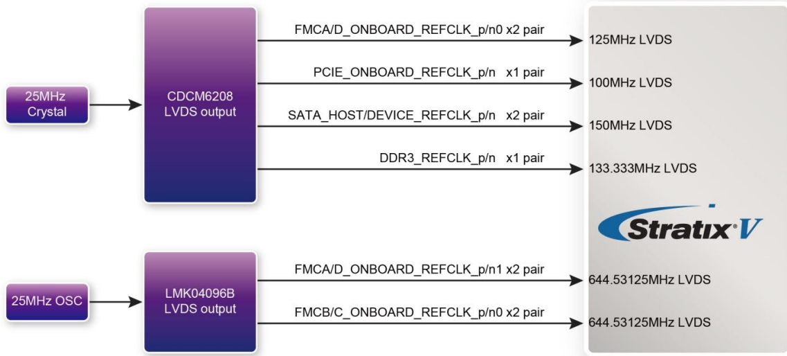
Figure 5-1 Programmable PLL Block diagram
