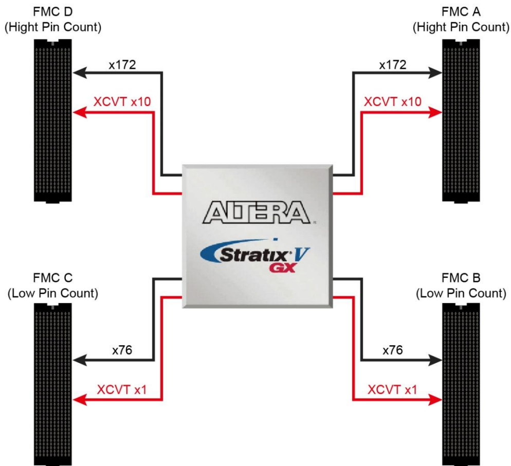
Figure 2-14 FMC connectors on TR5 board
