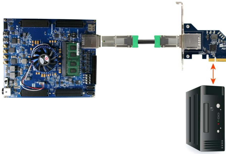
Figure 2-24 PCIe Link Setup between TR5 and PC
