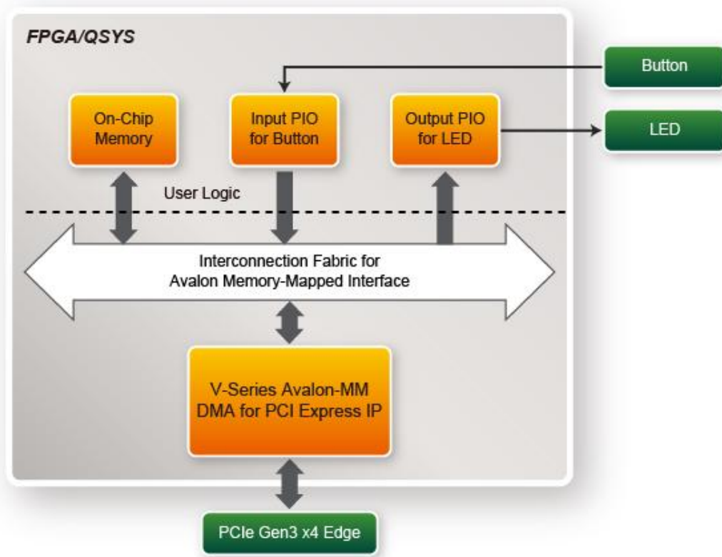
Figure 7-16 Hardware block diagram of the PCIe reference design
