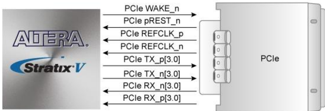
Figure 2-25 PCI Express Pin Connection
