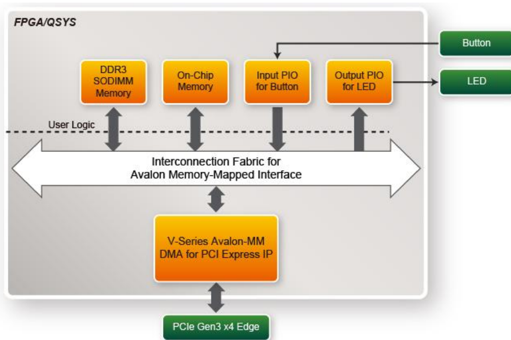
Figure 7-21 Hardware block diagram of the PCIe DDR3 reference design
