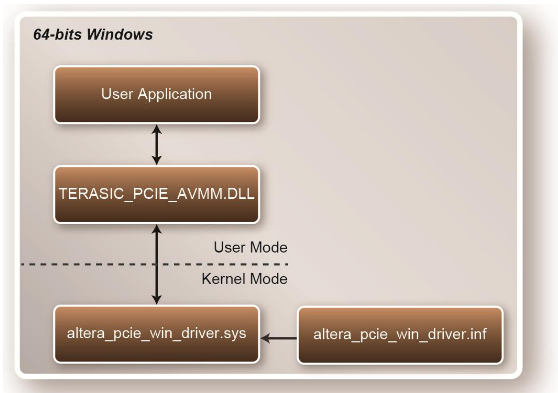
Figure 7-2 PCI Express Software Stack
