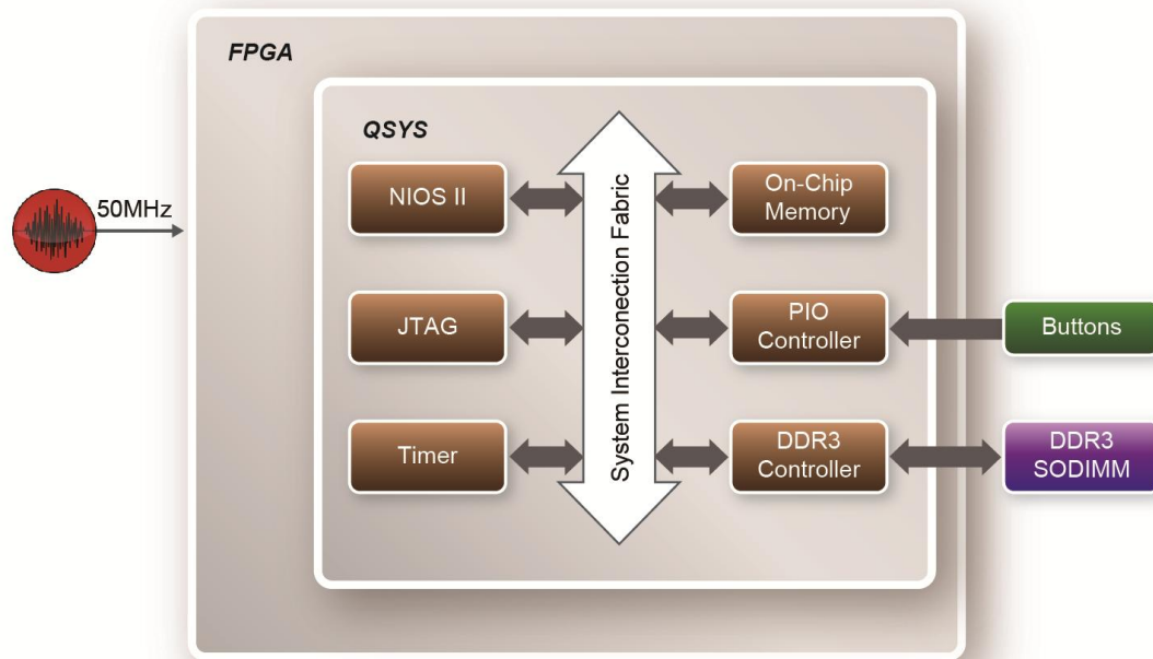
Figure 6-4 Block diagram of the DDR3 Basic Demonstration
