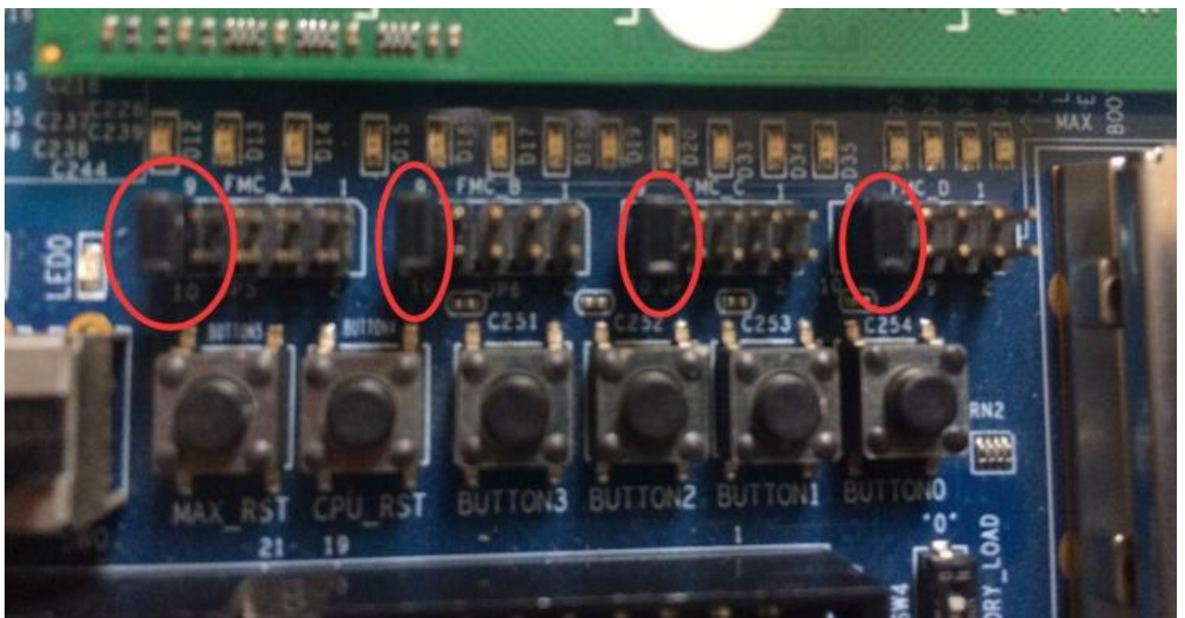
Figure 2-6 Set individual FMC connector VCCIO to 3.0V (Short Pin 9 & Pin 10 of JP5, JP6, JP7 and JP9)
