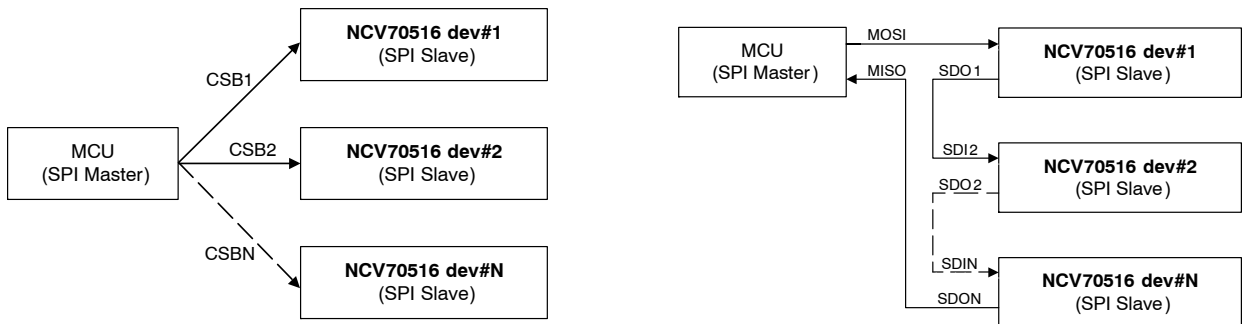
Figure 14. SPI Star vs. Daisy Chain Connection
