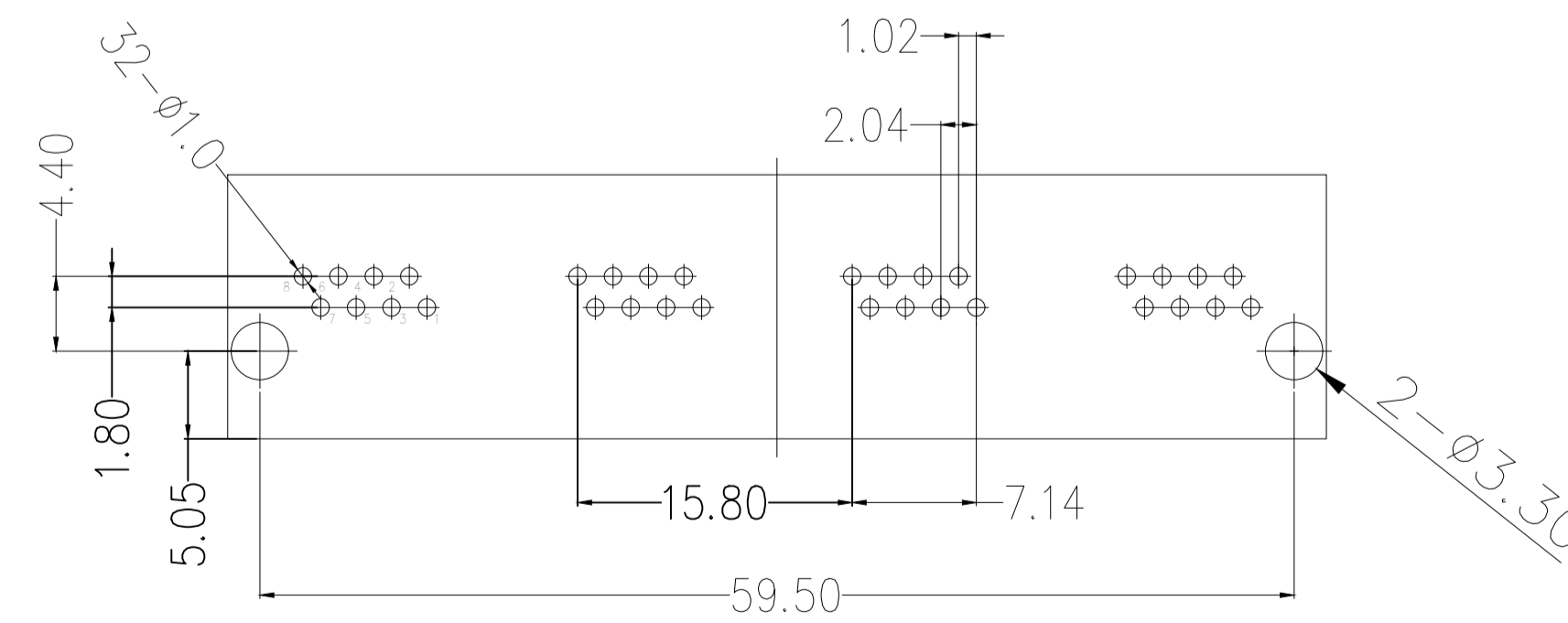
RECOMMENDER P.C.B.LAYOUT TOP VIEW (COMPONENT SIDE TOLERANCE \pm 0.05 )
