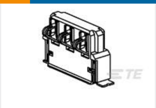
TE Part #1827928-1 LEAF BATTERY CONN 3POS. P=3.2,
