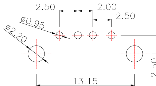
PCB.WELDING DRAWING (TOLERANCE:±0.05)
