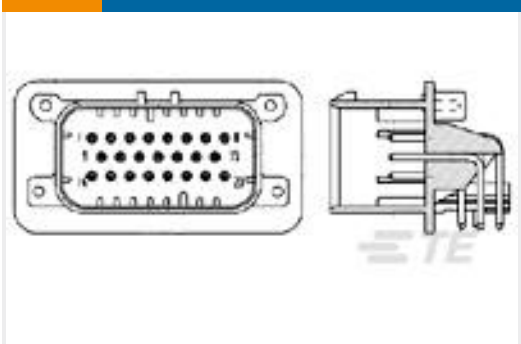
TE Part #1-776267-1 14POS,PIN DIA 1.3,HDR ASSY,90DEG, COD 1
