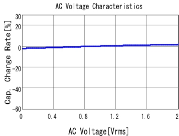
■ GRM188B11H102KA01 C-AC Voltage capchange, DC0V, 20.0d
