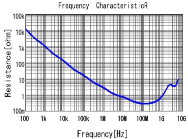
■ GRM188B11H102KA01 R DC0V, 20degC
