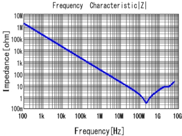
■ GRM188B11H102KA01 |Z| DC0V, 20degC
