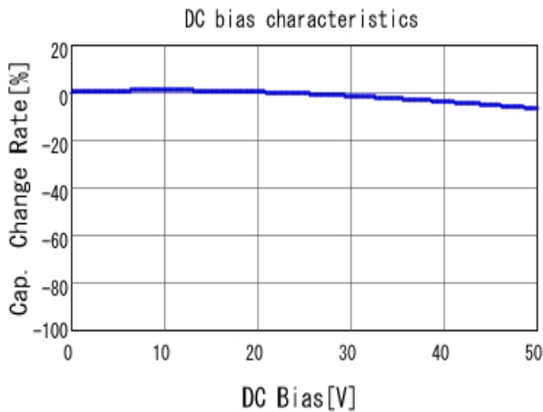
■ GRM188B11H102KA01 C-DC bias capchange, 20.0degC, AC1.
