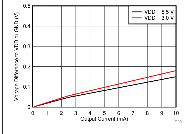
Figure 35. \overline{OR} Pin Trip Level vs Output Current
