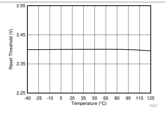
Figure 60. Power-On Reset Threshold vs Temperature
