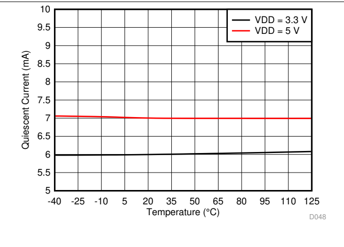
Figure 58. Quiescent Current vs Temperature
