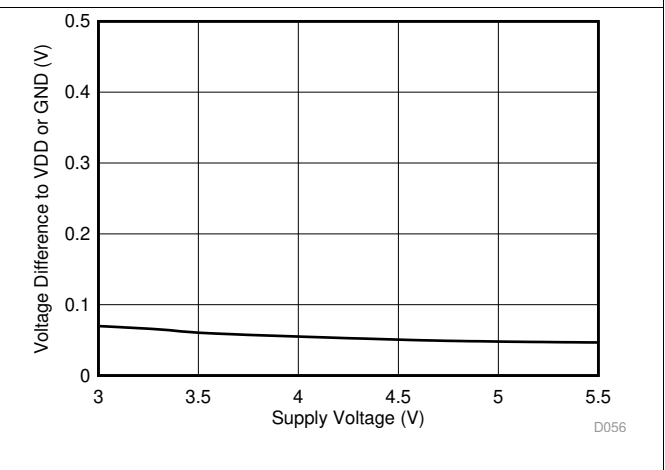
Figure 36. \overline{OR} Pin Trip Level vs Supply Voltage
