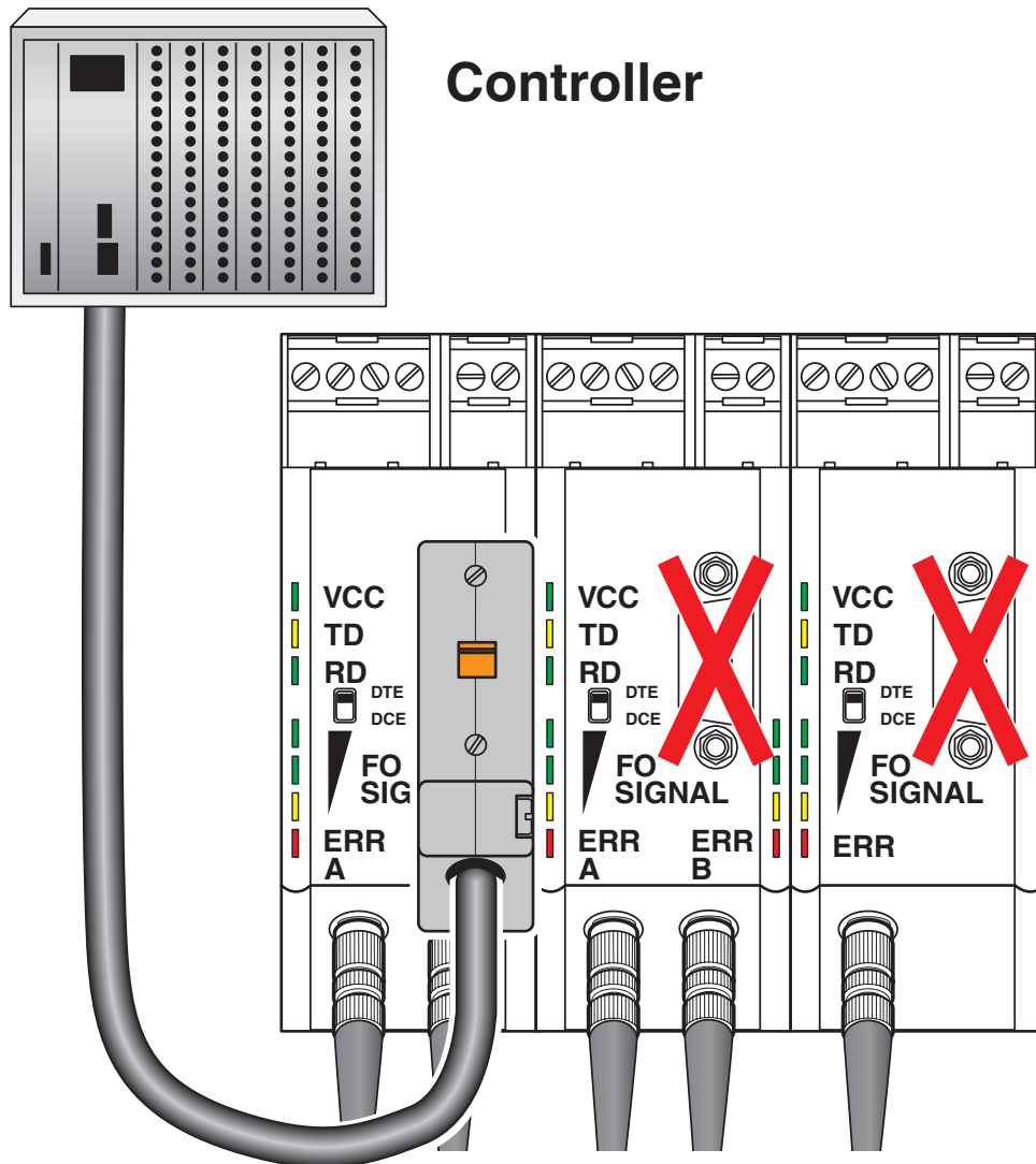
Schematic diagram
