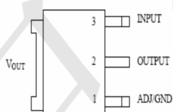
TO-252
