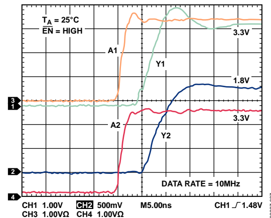
Figure 30. Normal Mode V_{CC1} = 3.3V , V_{CC2} = 1.8V
