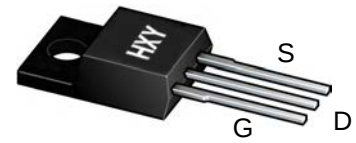
TO-220F (TO-220F-3L)
