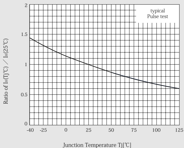
I_H - T_j 特性 Holding Current vs Junction Temperature
