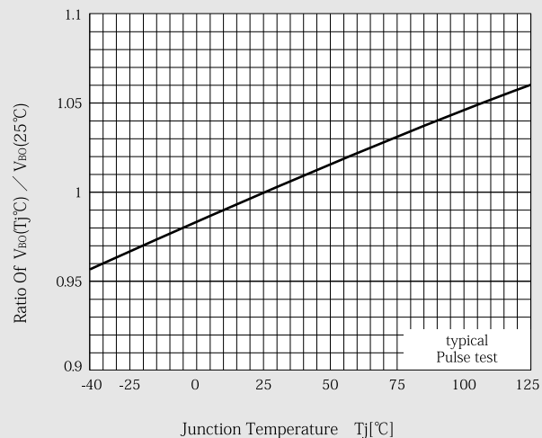
V_{BO} - T_j 特性 Break Over Voltage vs Junction Temperature
