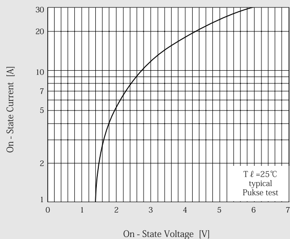
オン電圧－オン電流 On - State Voltage vs On - State Current
