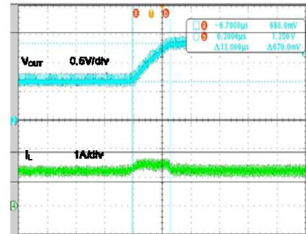
Dynamic Voltage Switch ( V_{IN}=6.0V , 0A Load, V_{OUT}=0.7125 \sim 1.5V , Slow Rate=12.5mV/19.2μs)
