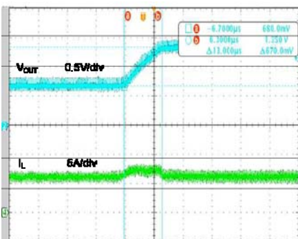
Dynamic Voltage Switch ( V_{IN}=6.0V , 8A Load, V_{OUT}=0.7125 \sim 1.5V , Slow Rate=12.5mV/0.15μs)
