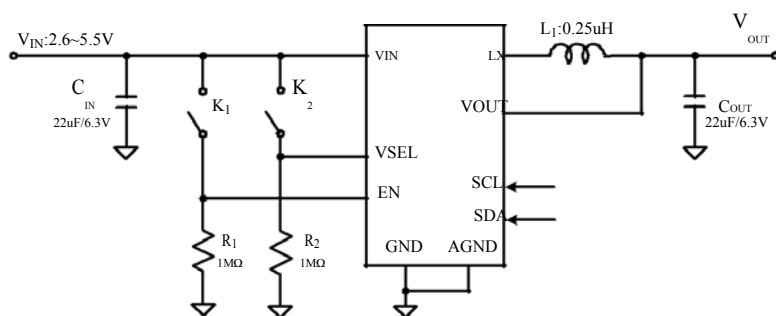
Figure 1. Schematic Diagram
