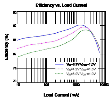
Figure2. Efficiency
