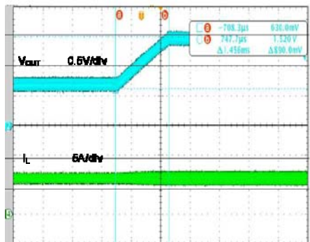
Dynamic Voltage Switch ( V_{IN}=6.0V , 8A Load, V_{OUT}=0.7125 \sim 1.5V , Slow Rate=12.5mV/19.2μs)
