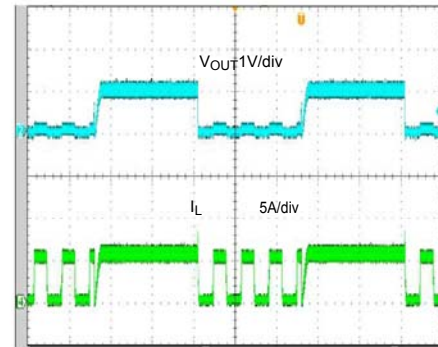
Short Circuit Protection ( V_{IN}=5.0V , V_{OUT}=1.0V , I_O=6A \sim \text{short} )
