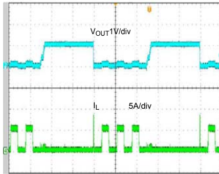
Short Circuit Protection ( V_{IN}=5.0V , V_{OUT}=1.0V , I_O=0A \sim \text{short} )
