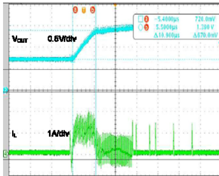
Dynamic Voltage Switch ( V_{IN}=6.0V , 0A Load, V_{OUT}=0.7125 \sim 1.5V , Slow Rate=12.5mV/0.15 \mu s )
