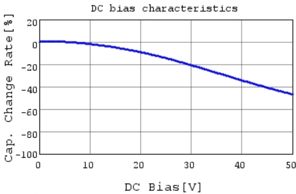
GCM155R71H682KA55 C-DC bias capchange, 25.0c
