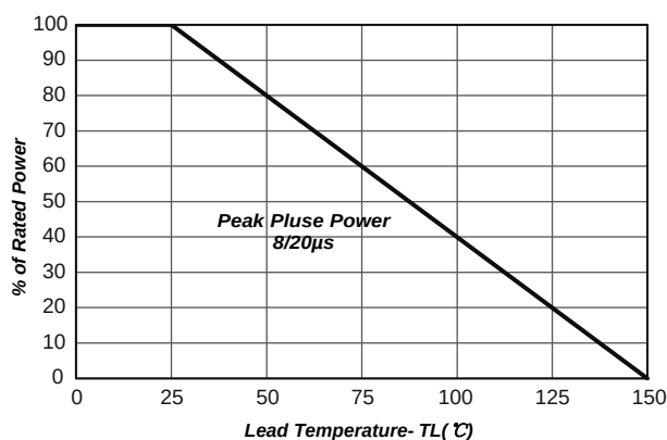
Fig2. Power Derating
