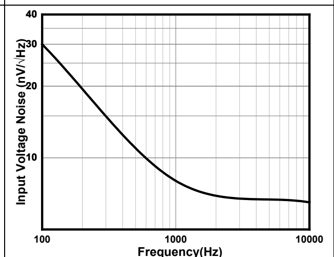
Figure 5. Input Voltage Noise Spectral Density
