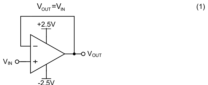
Figure 8. Voltage Follower
