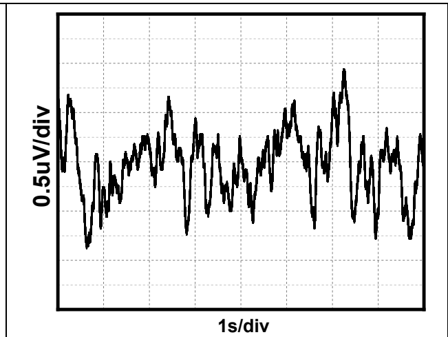
Figure 3. 0.1Hz to 10Hz Noise
