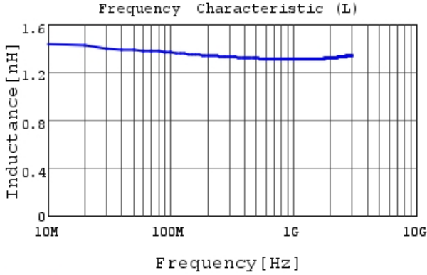
LQP03TN1N3B02 L
