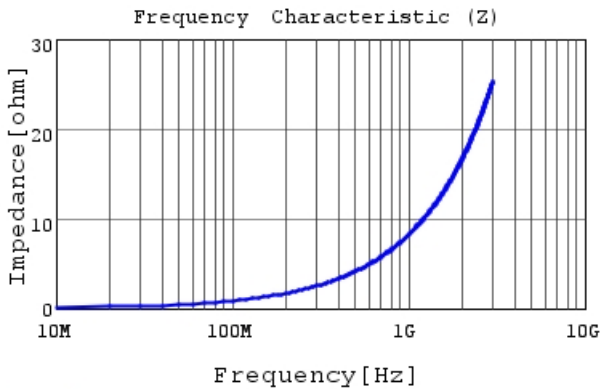
LQP03TN1N3B02 |Z|
