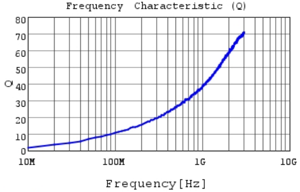
LQP03TN1N3B02 Q
