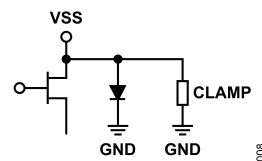
Figure 8. VSS Input Interface Schematic
