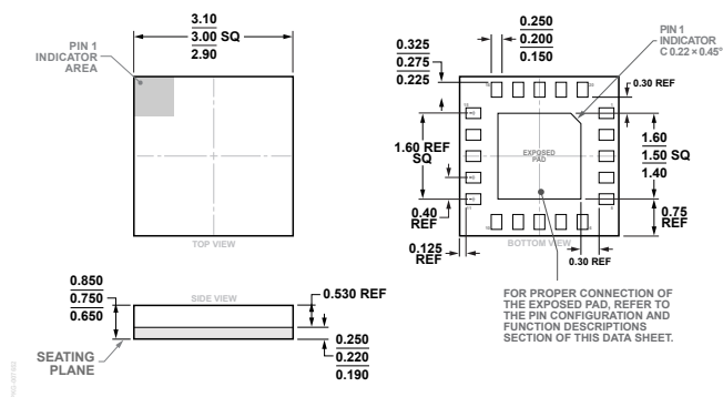
Figure 29. 20-Terminal Land Grid Array [LGA] (CC-20-9) Dimensions shown in millimeters
