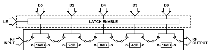
Figure 23. Simplified Circuit Diagram
