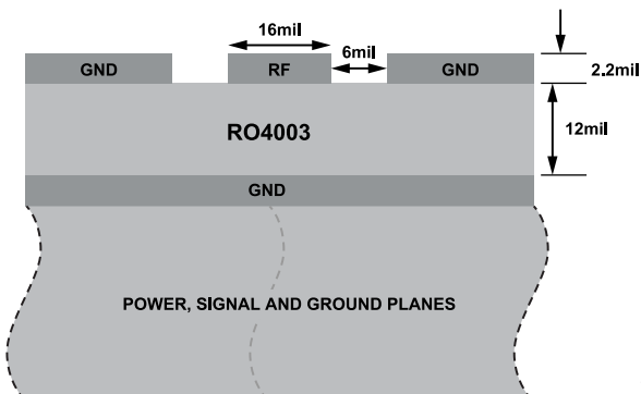
Figure 26. Example PCB Stackup
