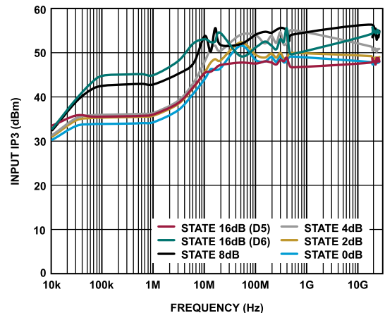
Figure 22. Input IP3 vs. Frequency, Low Frequency Detail
