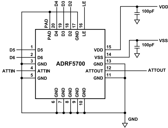
Figure 25. Recommended Schematic
