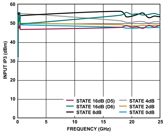
Figure 20. Input IP3 vs. Frequency
