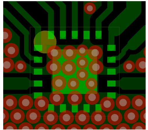
Figure 27. PCB Routings
