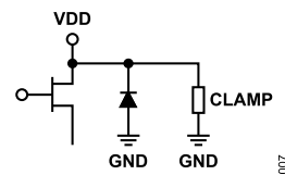
Figure 7. VDD Input Interface Schematic
