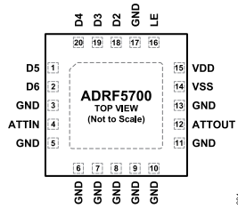
Figure 4. Pin Configuration
