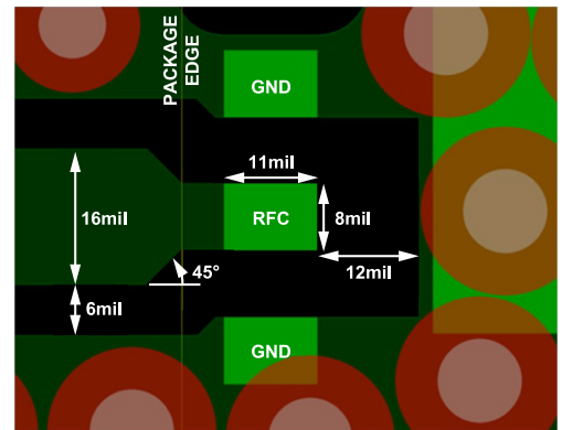
Figure 28. Recommended RF Pin Transitions
