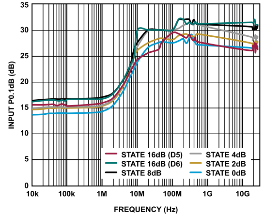
Figure 21. Input P0.1dB vs. Frequency, Low Frequency Detail
