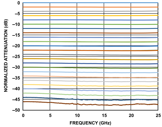
Figure 12. Normalized Attenuation vs. Frequency for All States
