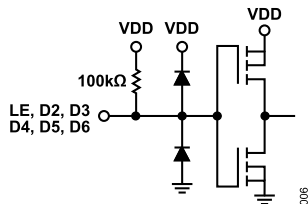
Figure 6. Digital Input Interface Schematic (LE, D2, D3, D4, D5, and D6)
