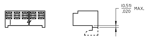
HOOKS CUT OPTION AVAILABLE ON TOP ENTRY. SEE CHART
