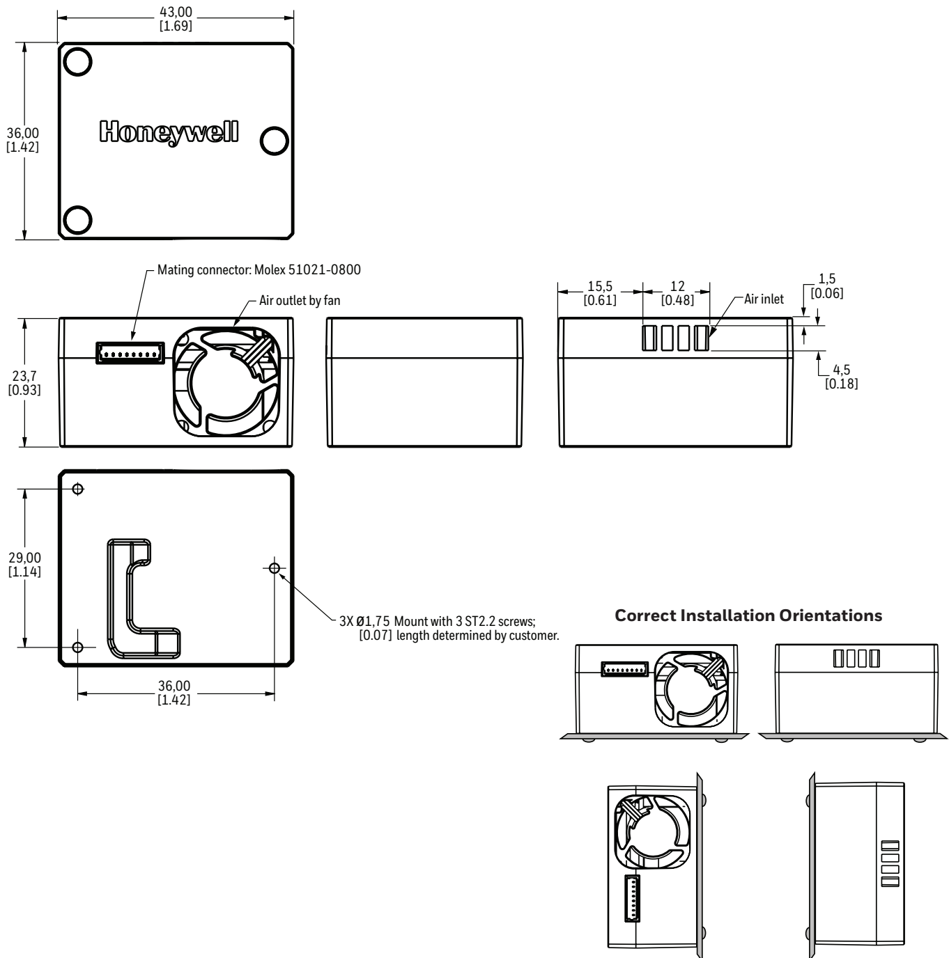
Figure 2. Standard Mounting Dimensions and Correct Installation Orientations (For reference only. (mm/[in])
