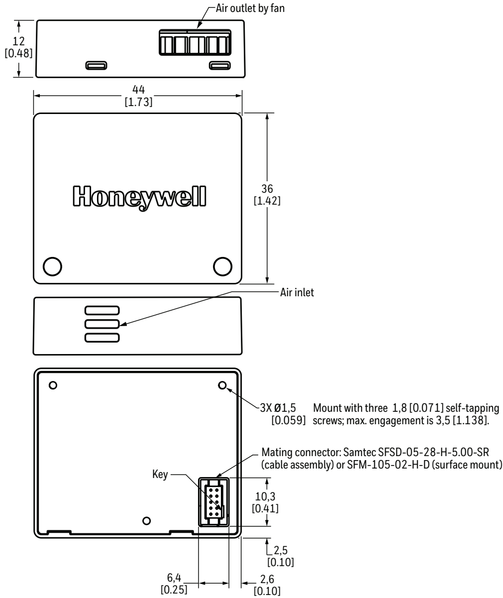
Figure 4. Compact Version HPMA115CO-002 Mounting Dimensions and Correct Installation Orientations (For reference only: mm/[in])
