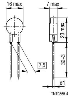
Dimensions in mm Approx. weight 3 g
