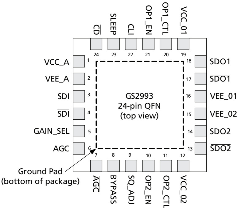
Figure 1-1: GS2993 Pin Assignment
