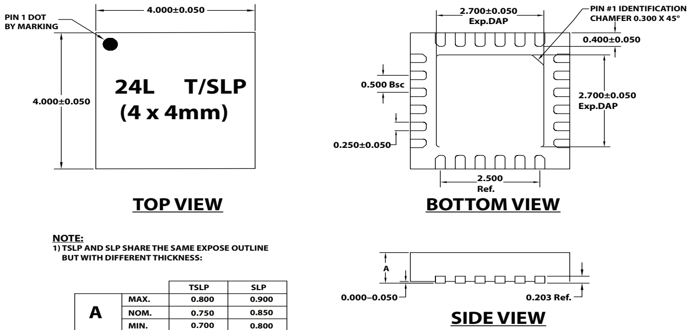
Figure 6-1: Package Dimensions
