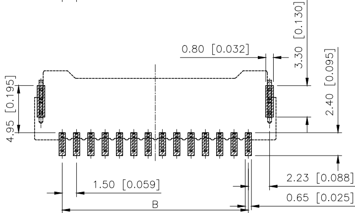
PCB LAYOUT
