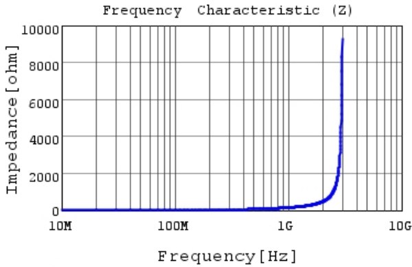
LQP03TN22NH02 |Z|
