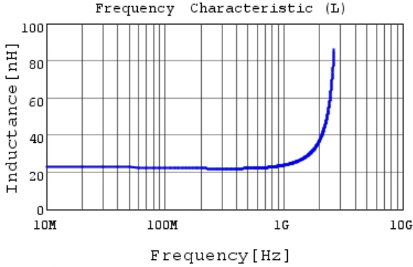
LQP03TN22NH02 L
