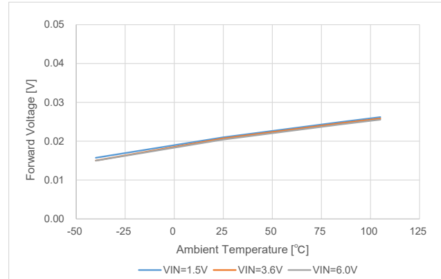
(6-2-1) Forward Voltage vs Ambient Temperature
