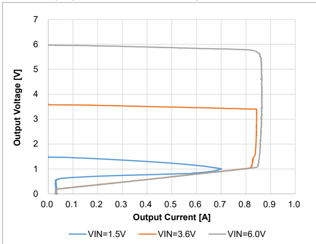
(10-1-2) Output Voltage vs Output Current
