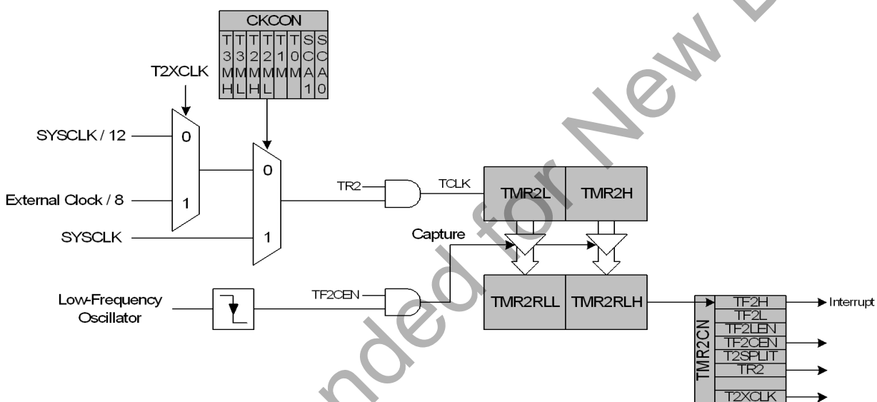
Figure 28.6. Timer 2 Low-Frequency Oscillation Capture Mode Block Diagram
