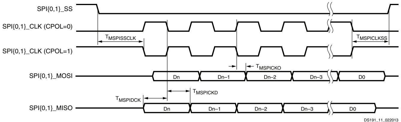
Figure 13: SPI Master (CPHA = 1) Interface Timing Diagram
