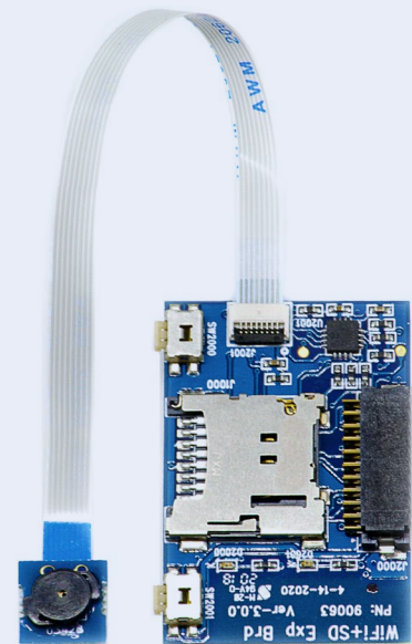
Add-On Board with optional Chirp Ultrasonic Time-of-Flight Sensor
