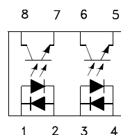
Internal connection diagram
