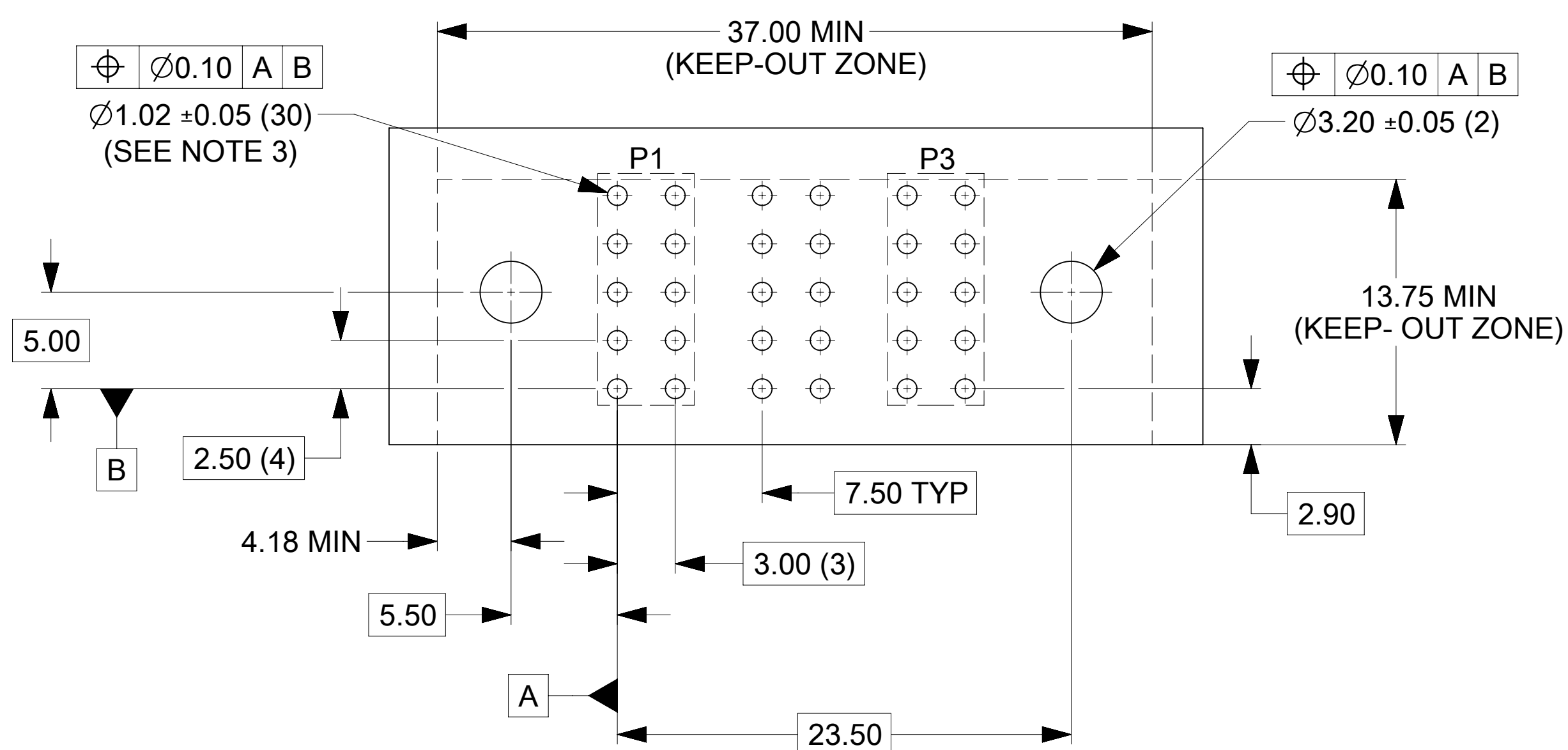
RECOMMENDED PCB LAYOUT AND KEEP-OUT ZONE
