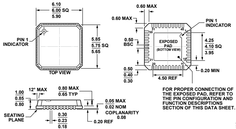
Figure 111. 40-Lead Lead Frame Chip Scale Package [LFCSP] 6 mm × 6 mm and 0.85 mm Package Height (CP-40-1) Dimensions shown in millimeters
