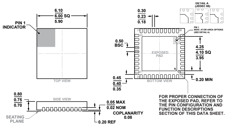
Figure 112. 40-Lead Lead Frame Chip Scale Package [LFCSP] 6 mm × 6 mm and 0.75 mm Package Height (CP-40-9) Dimensions shown in millimeters
