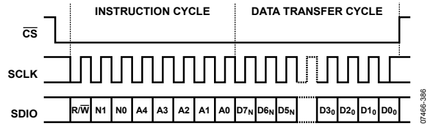
Figure 86. Serial Register Interface Timing, MSB First Read
