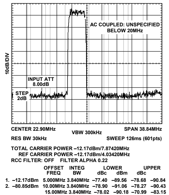
Figure 65. AD9117 ACLR One-Carrier, 3.3 V
