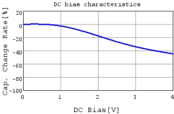
NFM18HC106D0G3 C-DC bias capchange, 25.0degC
