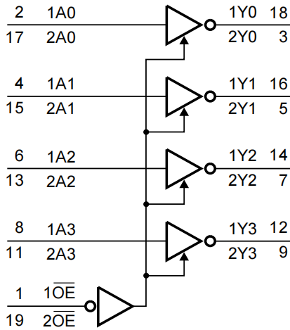
Figure 1. Logic symbol
