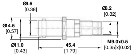
Part No. 1-1393665-5 ♦
