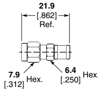
Part No. 1060494-1
