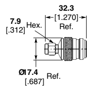
Part No. 1058664-1
