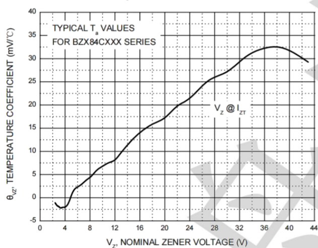
Temperature Coefficients
