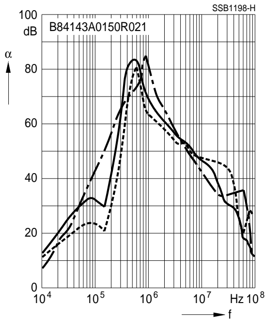
Filters for 150 A
