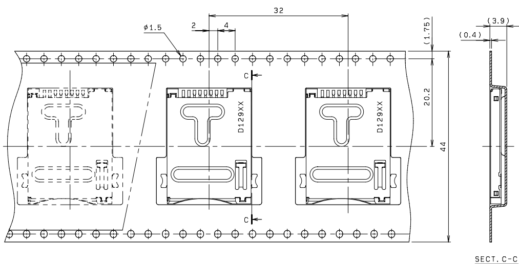
SECT. C-C
