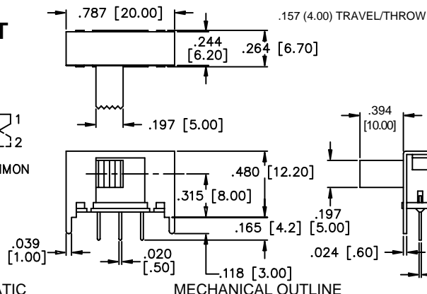
MECHANICAL OUTLINE
