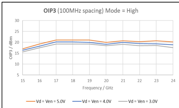
Figure 23: OIP3 100MHz spacing, P_{out} = -7\text{dBm/ton} , high current mode
