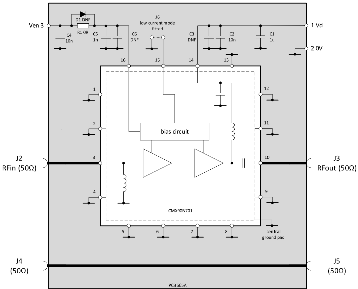
Figure 62: EV90B701 Schematic
