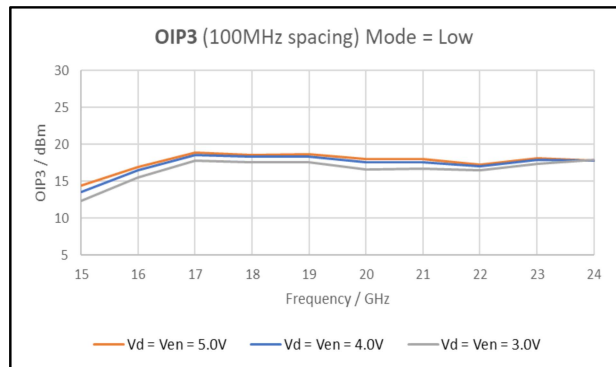
Figure 24: OIP3 100MHz spacing, P_{out} = -7\text{ dBm/ton} , low current mode
